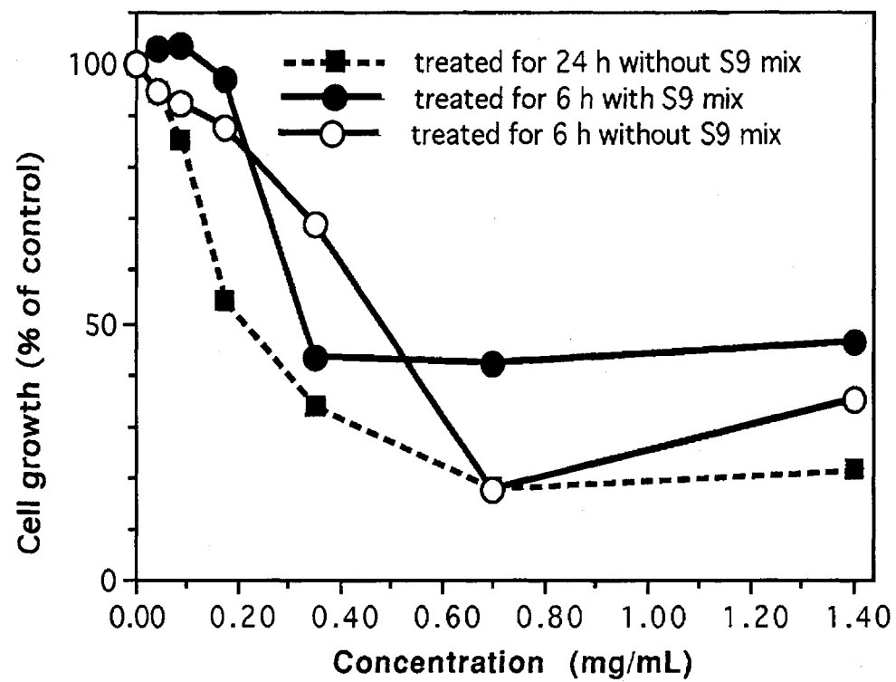
Fig. 1 Growth inhibition of CHL/IU cells treated with 4-(1-methylethyl) aniline
