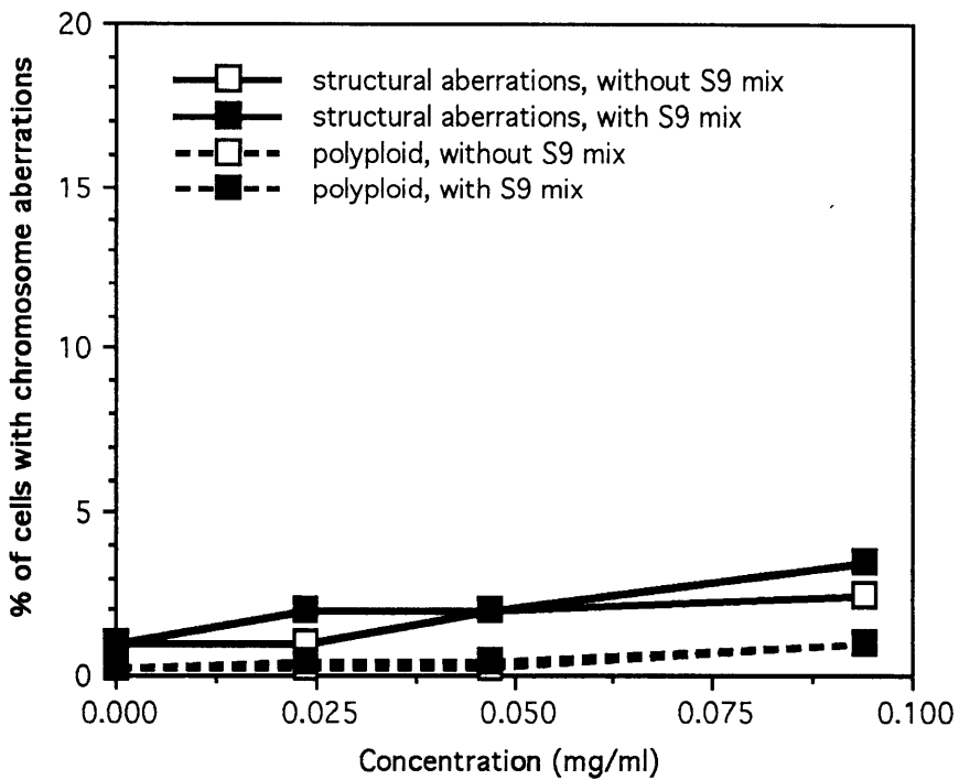
Fig. 3 Induction of chromosome aberrations in CHL cells treated with 1,4-dichloro-2-nitrobenzene with and without S9 mix
