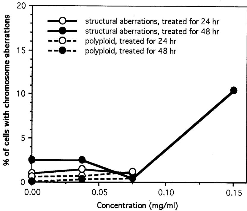
Fig. 2 Induction of chromosome aberrations in CHL cells continuously treated with 1,4-dichloro-2-nitrobenzene without S9 mix
