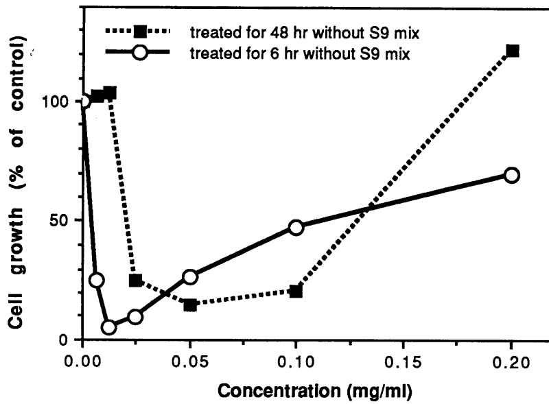
Fig.1 Inhibition of cell growth treated with triisobutylene without S9 mix in CHL cells
