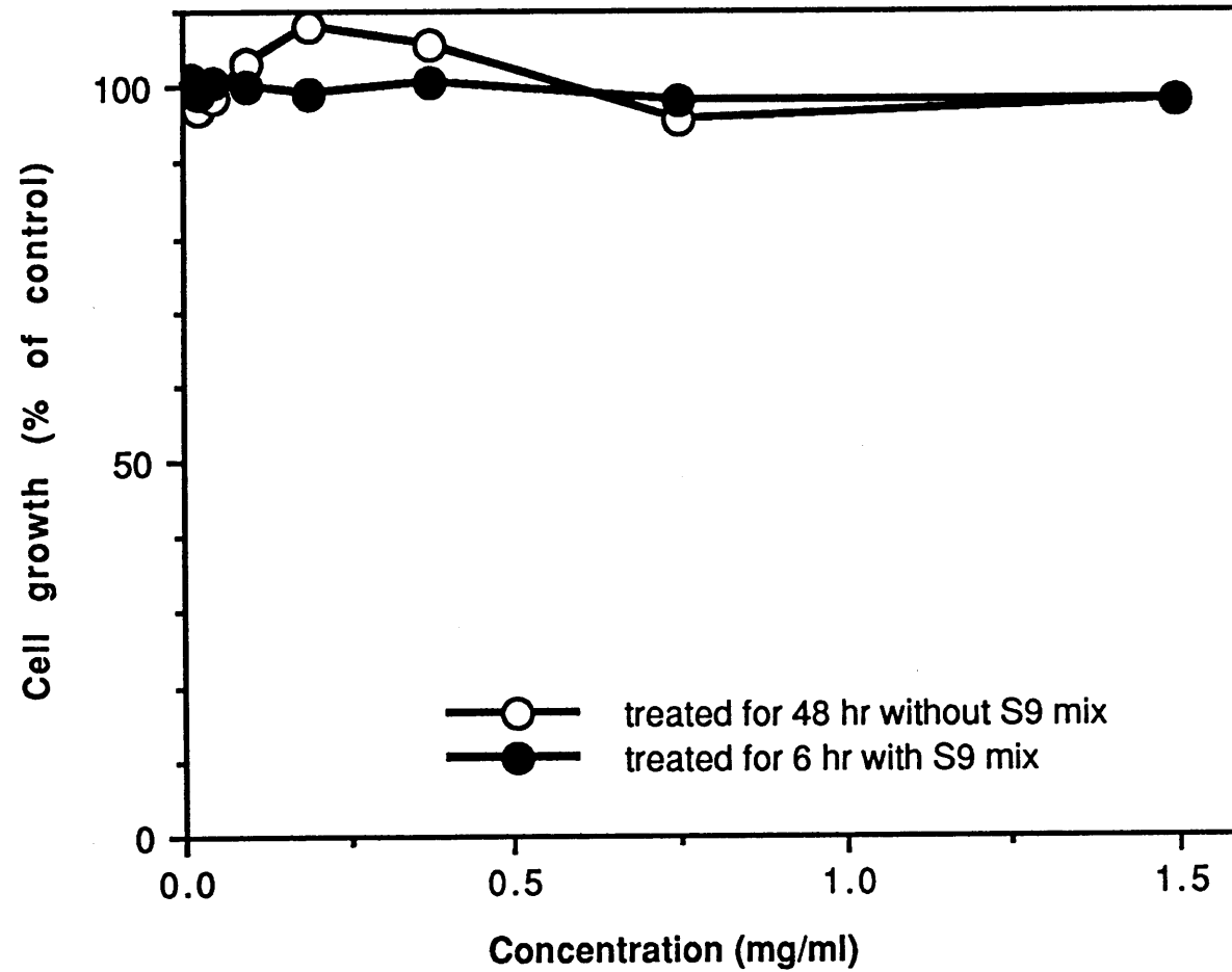
Fig. 1 Inhibition of cell growth treated with 2-ethyl-2-hydroxymethyl-1,3-propanediol in CHL cells
