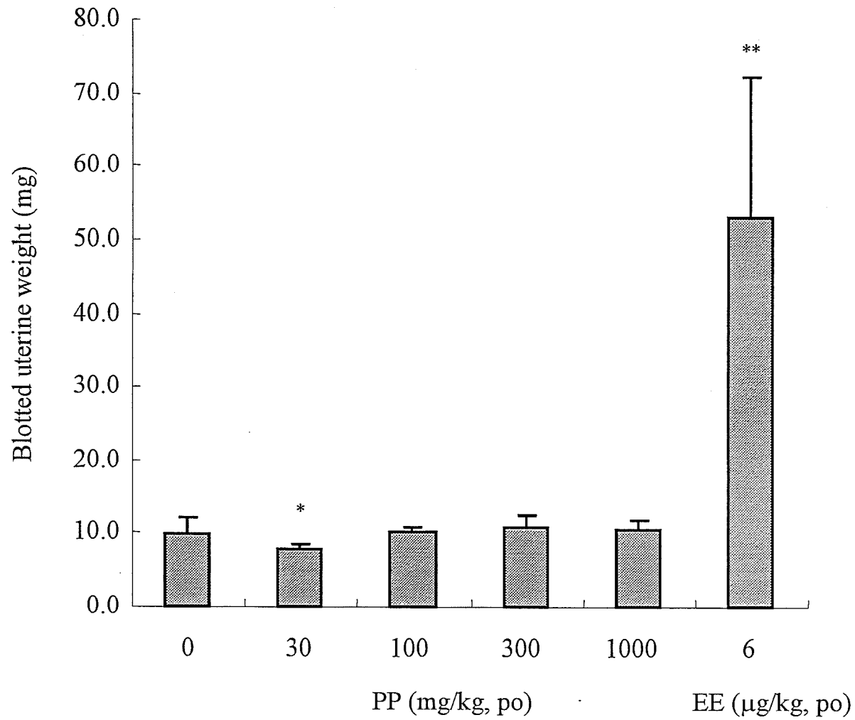
Fig. 1 Uterotrophic assay of PP for estrogenic activity detection in ovariectomized C57BL/6J mice
