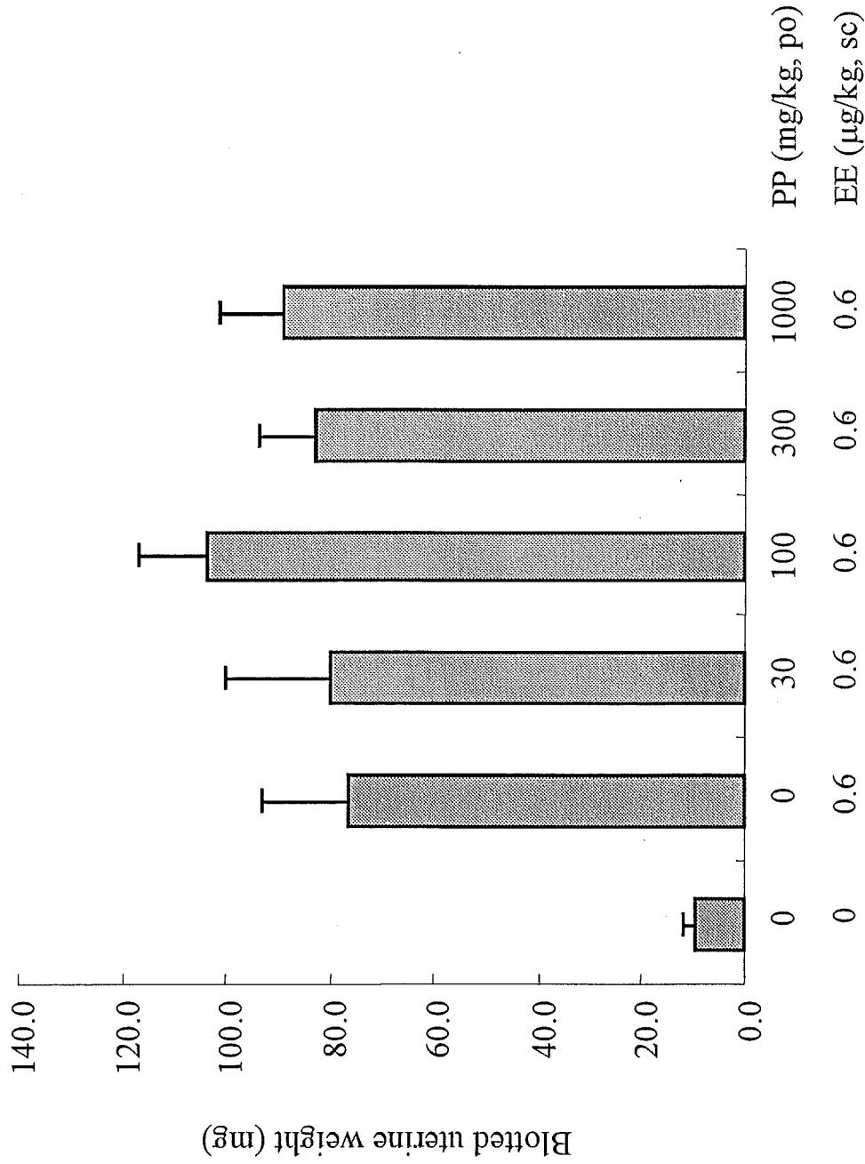
Fig. 2 Uterotropic assay of PP for antiestrogenic activity detection in ovariectomized C57BL/6J mice
