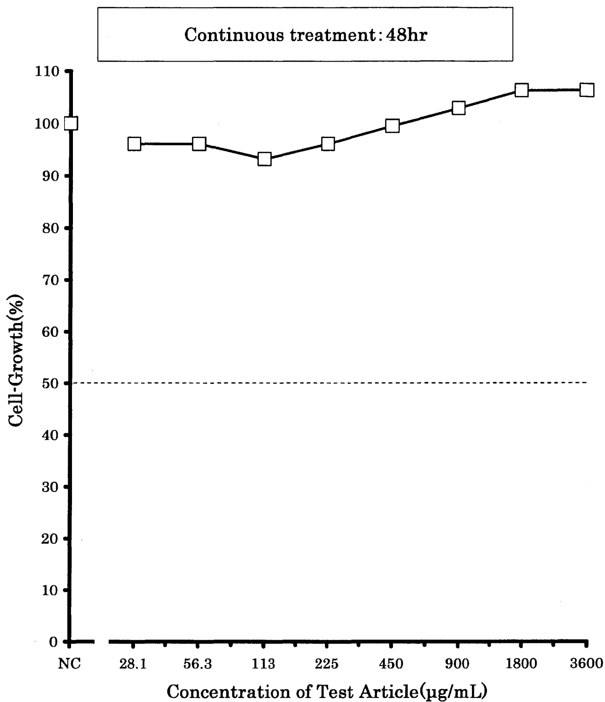
Fig.1-4 Results of the cell-growth inhibition test in cultured Chinese hamster cells treated with 2-(2H-benzotriazol-2-yl)-4,6-di-tert-pentylphenol
