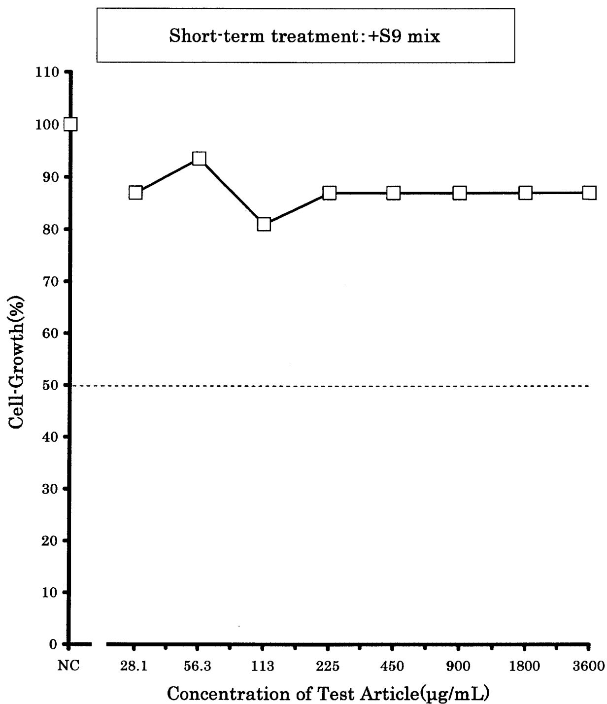
Fig.1-1 Results of the cell-growth inhibition test in cultured Chinese hamster cells treated with 2-(2H-benzotriazol-2-yl)-4,6-di-tert-pentylphenol
