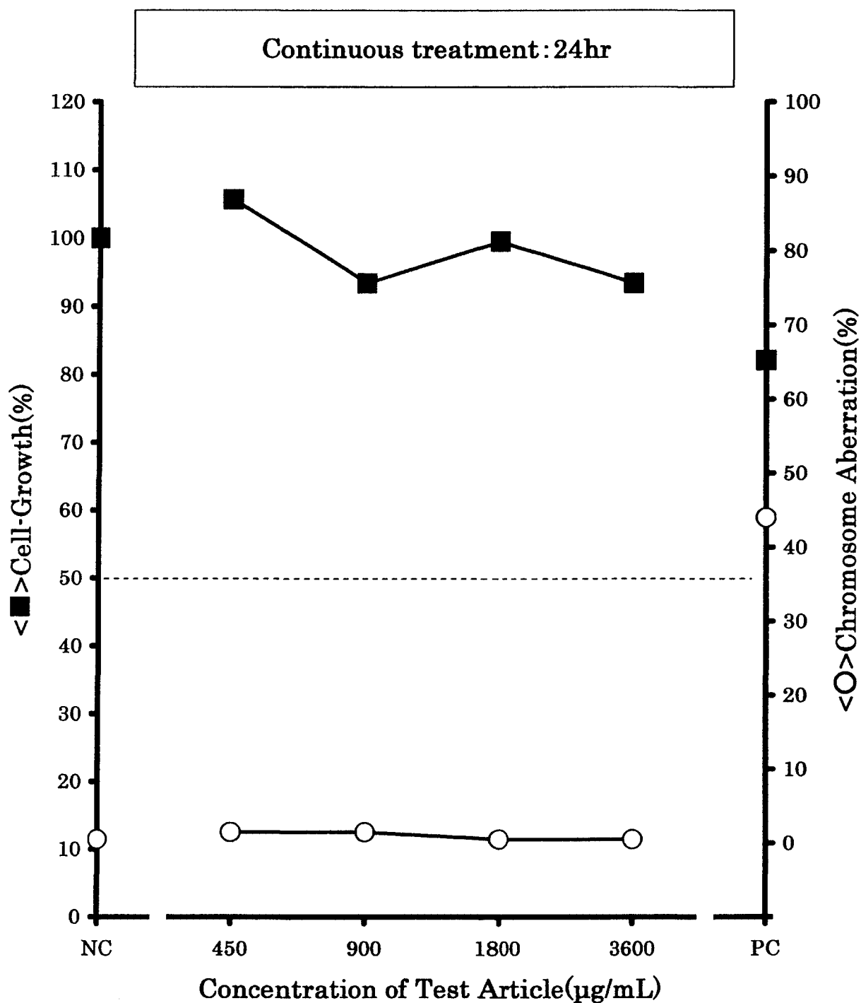
Fig.2-3 Results of the chromosome aberration test in cultured Chinese hamster cells treated with 2-(2H-Benzotriazol-2-yl)-4,6-di-tert-pentylphenol
