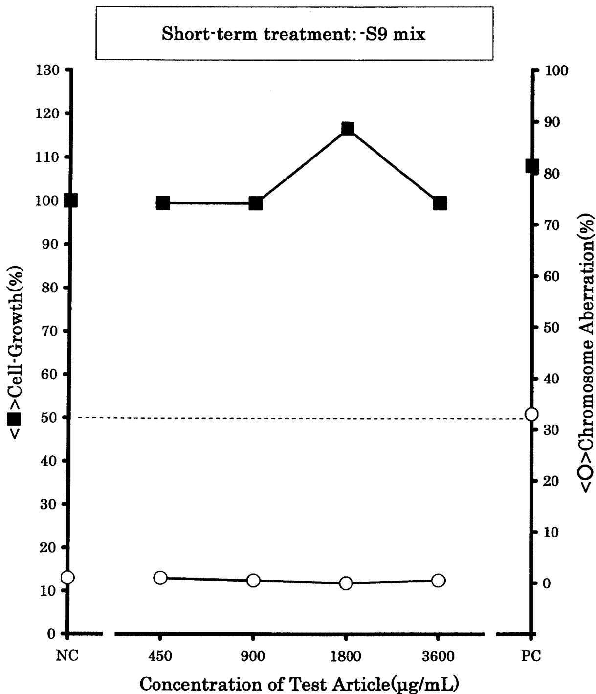
Fig.2-2 Results of the chromosome aberration test in cultured Chinese hamster cells treated with 2-(2H-Benzotriazol-2-yl)-4,6-di-tert-pentylphenol
