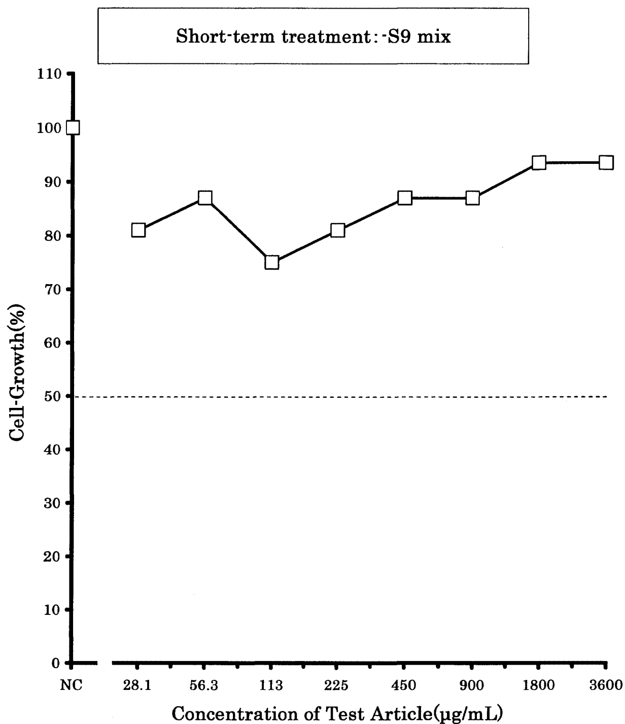
Fig.1-2 Results of the cell-growth inhibition test in cultured Chinese hamster cells treated with 2-(2H-benzotriazol-2-yl)-4,6-di-tert-pentylphenol
