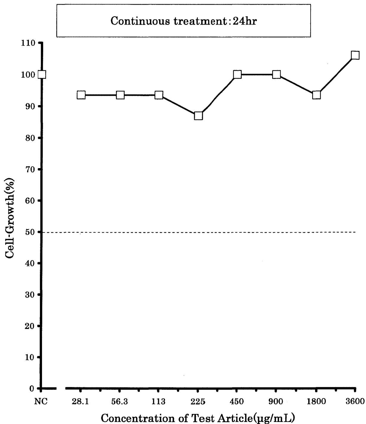
Fig.1-3 Results of the cell-growth inhibition test in cultured Chinese hamster cells treated with 2-(2H-benzotriazol-2-yl)-4,6-di-tert-pentylphenol
