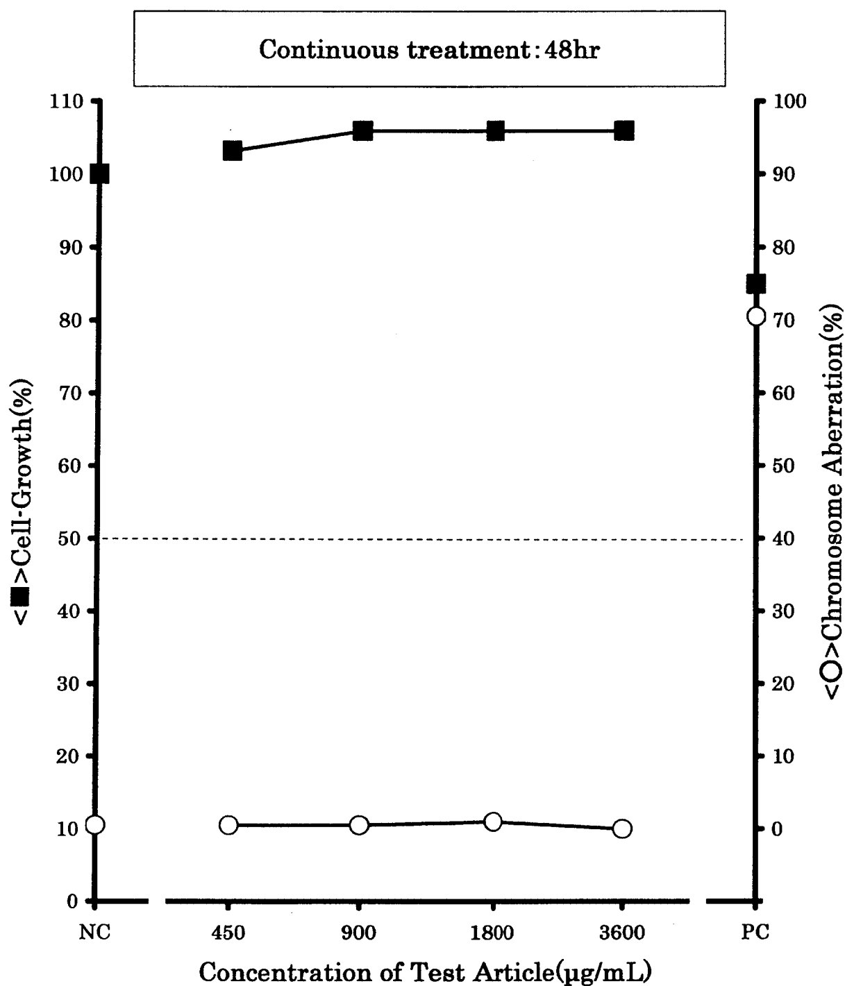
Fig.2-4 Results of the chromosome aberration test in cultured Chinese hamster cells treated with 2-(2H-Benzotriazol-2-yl)-4,6-di-tert-pentylphenol
