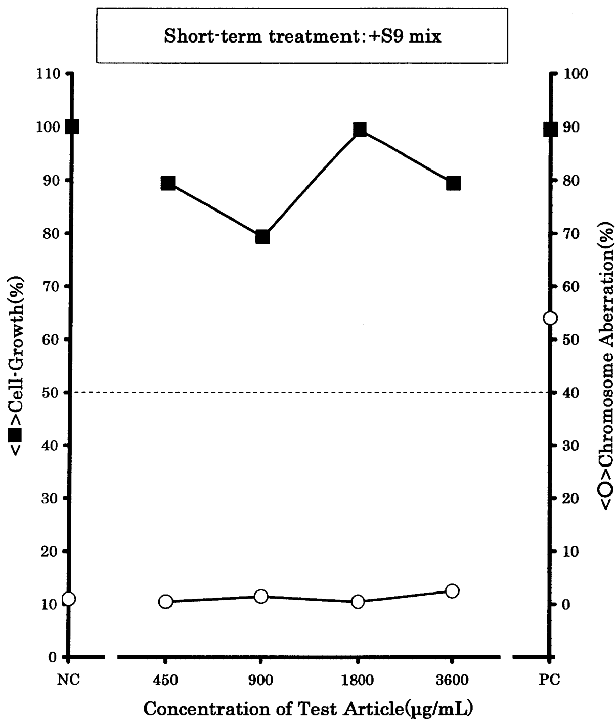
Fig.2-1 Results of the chromosome aberration test in cultured Chinese hamster cells treated with 2-(2H-Benzotriazol-2-yl)-4,6-di-tert-pentylphenol
