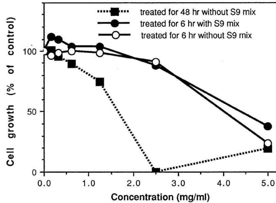
Fig.1 Inhibition of cell growth treated with 3-aminobenzenesulfonic acid in CHL cells
