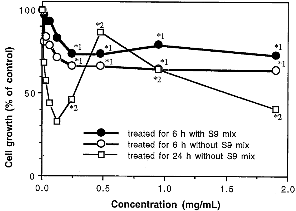
Fig.1 Growth inhibition of CHL/IU cells treated with 4,4'-biphenyldiol
