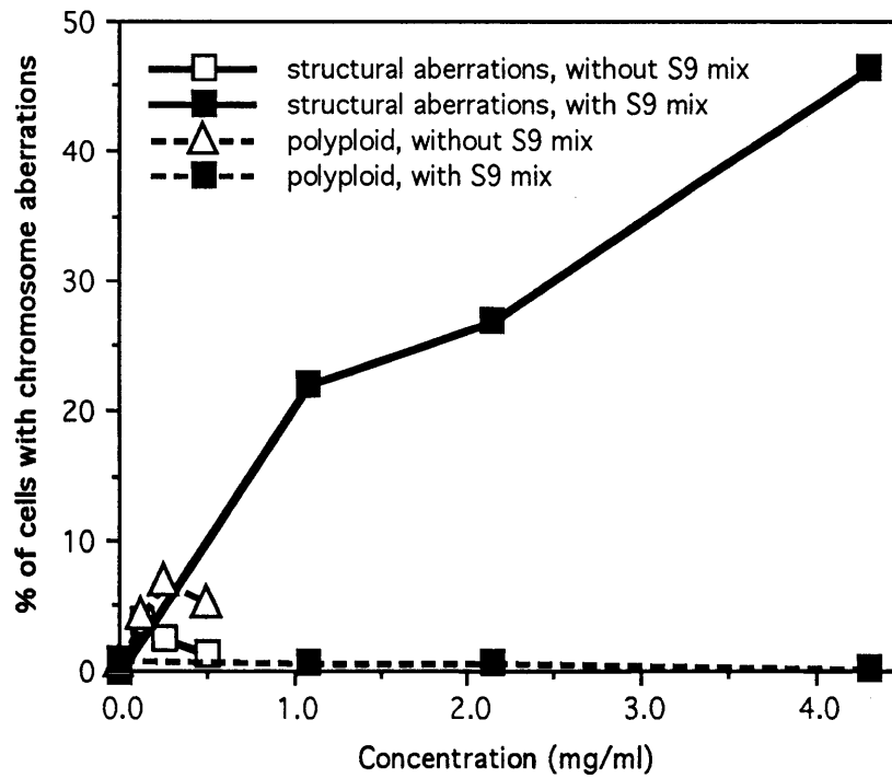
Fig. 3 Induction of chromosome aberrations in CHL/IU cells treated with sorbitan monooleate with and without S9 mix
