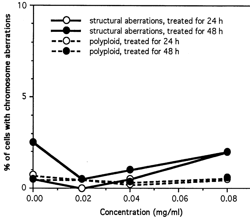
Fig. 2 Induction of chromosome aberrations in CHL/IU cells continuously treated with sorbitan monooleate without S9 mix
