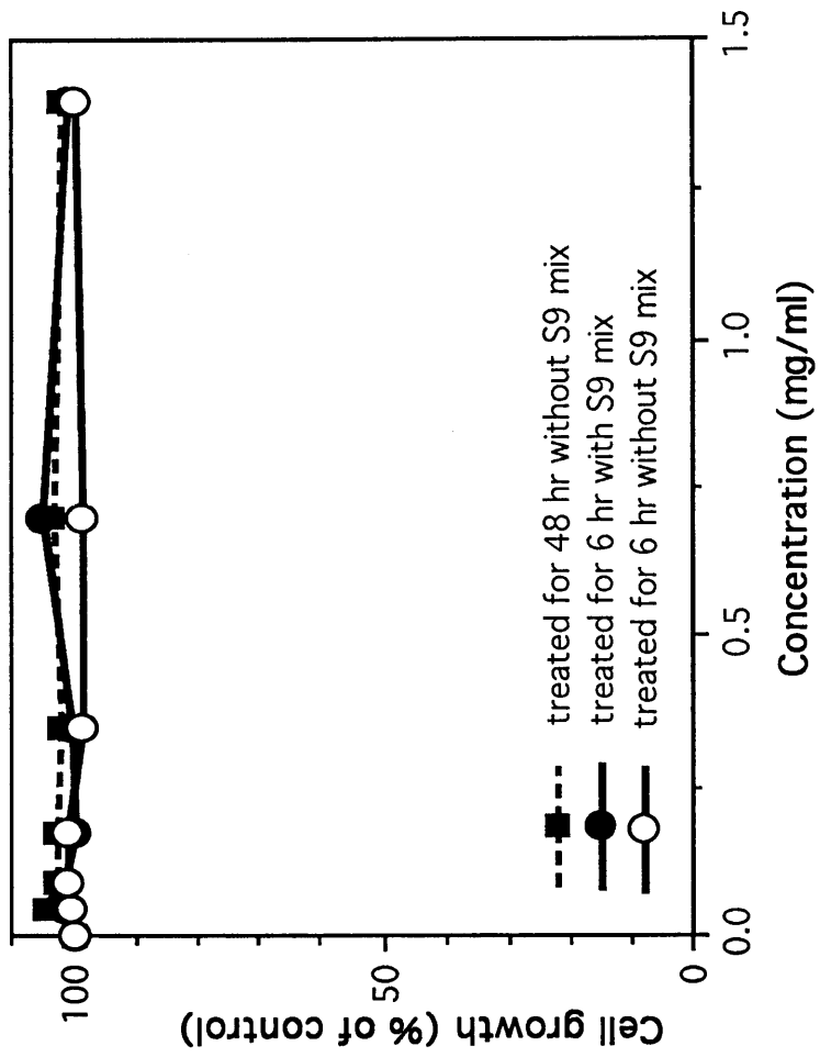
Fig.1 Growth inhibition of CHL cells treated with pentaerythritol
