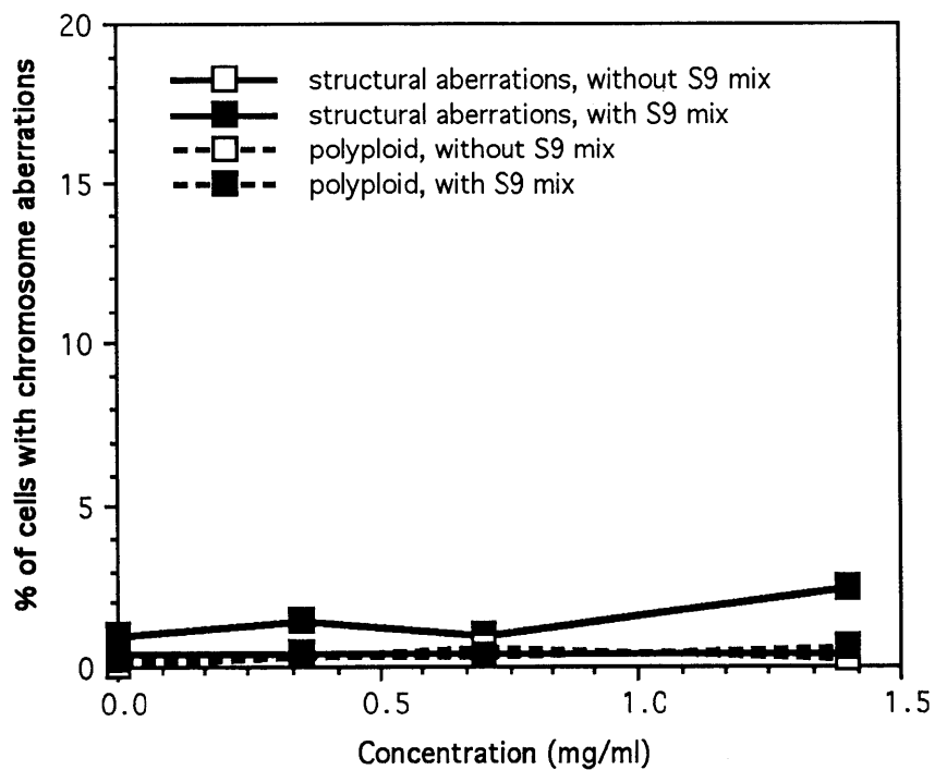
Fig. 3 Induction of chromosome aberrations in CHL cells treated with pentaerythritol with and without S9 mix
