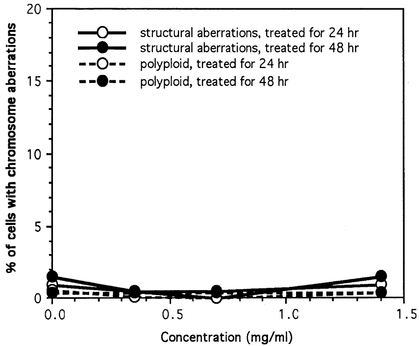
Fig. 2 Induction of chromosome aberrations in CHL cells continuously treated with pentaerythritol without S9 mix
