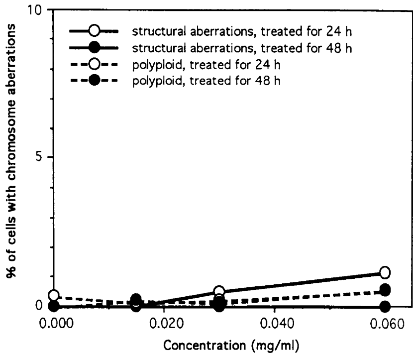
Fig. 2 Induction of chromosome aberrations in CHL/IU cells continuously treated with methyl dodecanoate without S9 mix
