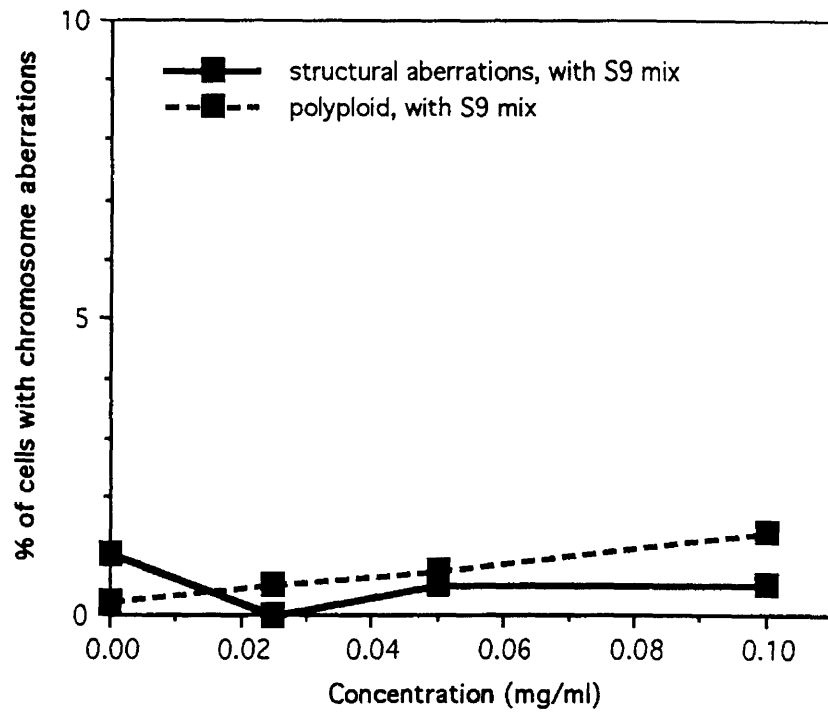
Fig. 4 Induction of chromosome aberrations in CHL/IU cells treated with methyl dodecanoate with S9 mix
