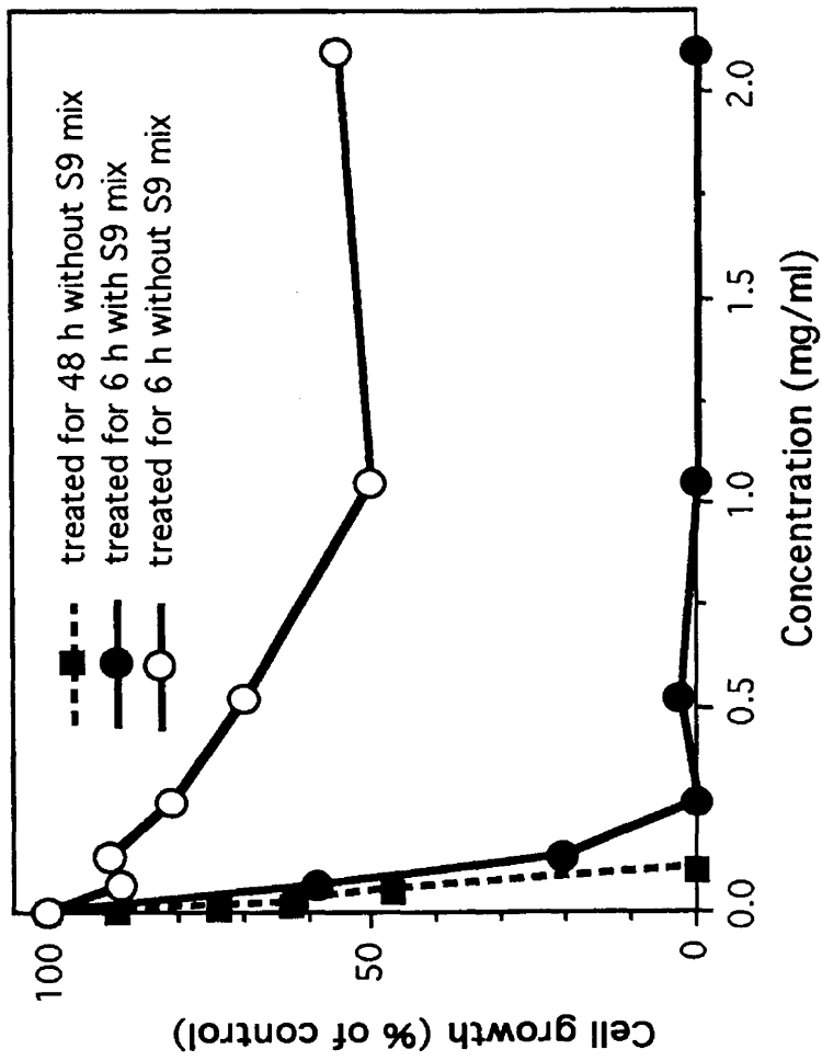
Fig. 1 Growth inhibition of CHL/IU cells treated with methyl dodecanoate
