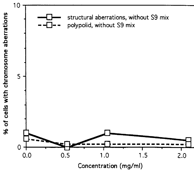
Fig. 3 Induction of chromosome aberrations in CHL/IU cells treated with methyl dodecanoate for 6 h without S9 mix
